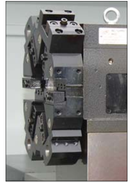
Optional 6-position turret
